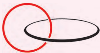
(a) 索烃
